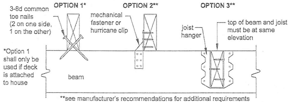
Figure 6: Joist-to-Beam Detail
