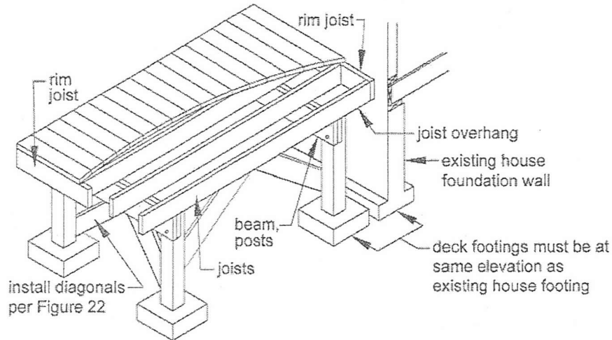
Figure 21: Free-Standing Deck
